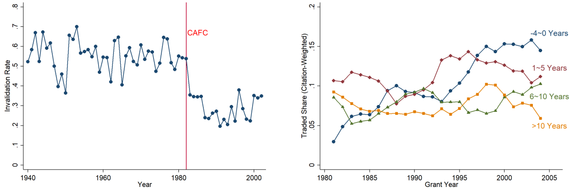
(a) Patent Invalidation Rates in Lawsuits (b) Patent Trade by Gaps from the Grant Year
